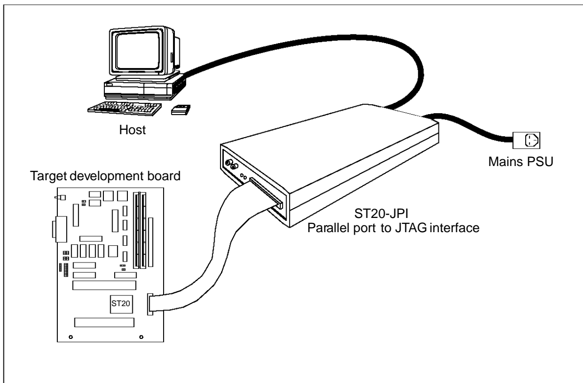
Figure 2.1 ST20-JPI connections basic configuration
