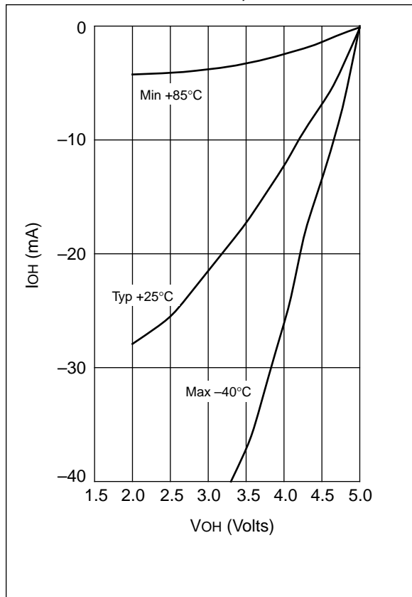
FIGURE 18-21: I_{OH} vs. V_{OH} , V_{DD} = 5\text{ V}
