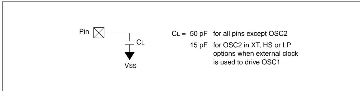
FIGURE 15-1: LOAD CONDITIONS
